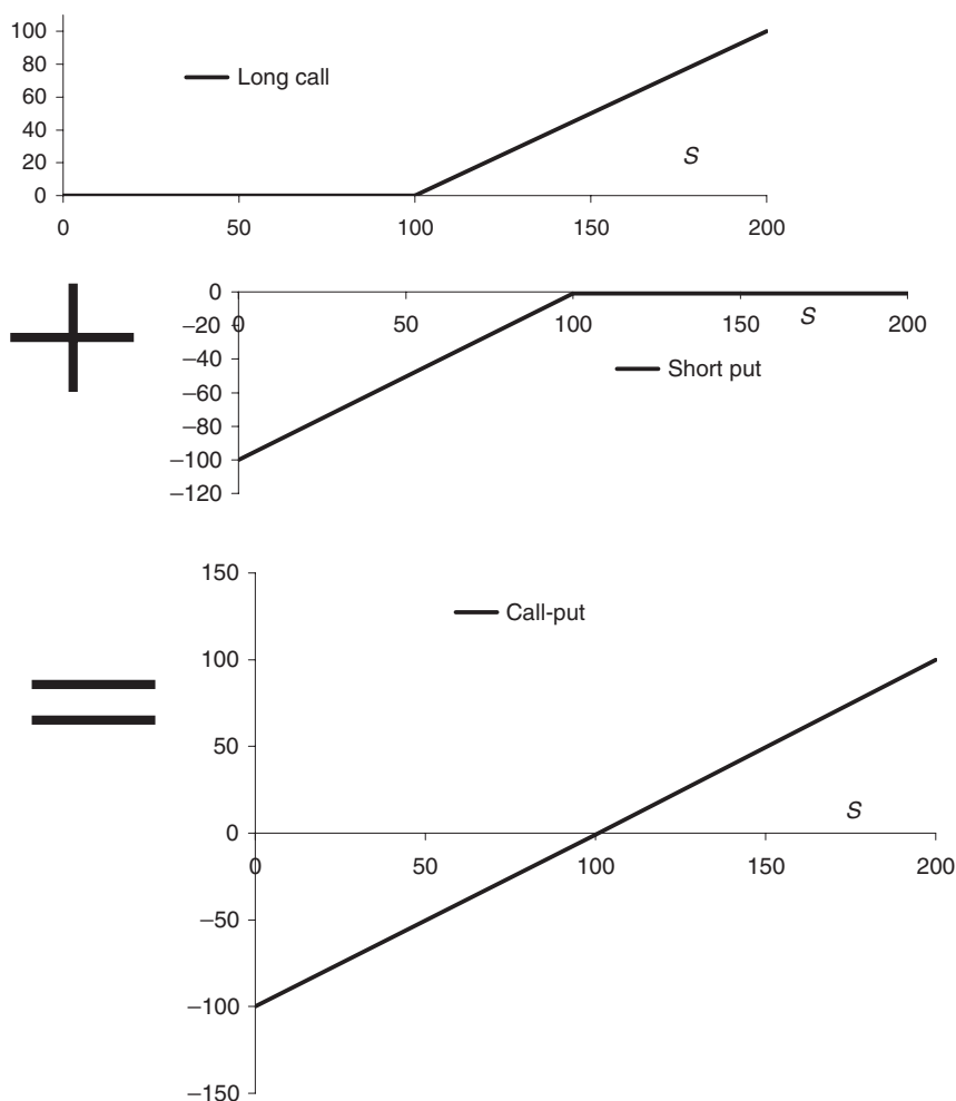
Figure 2.14 Schematic diagram showing put-call parity.
