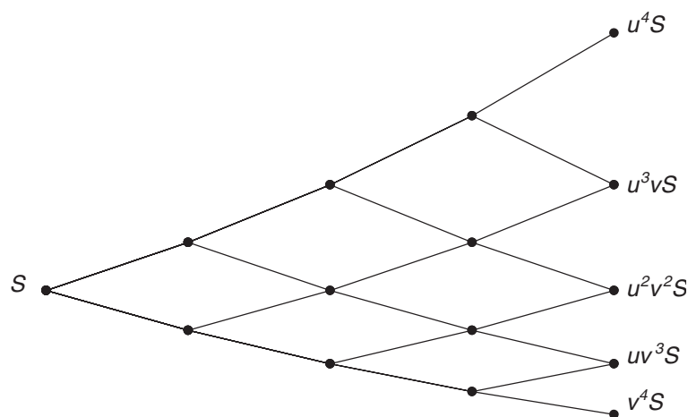
Figure 3.21 The binomial tree.
