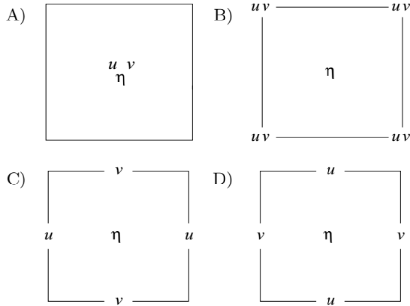
Figure 7.1: Four natural arrangements of shallow water variables on quadrilateral grids.
