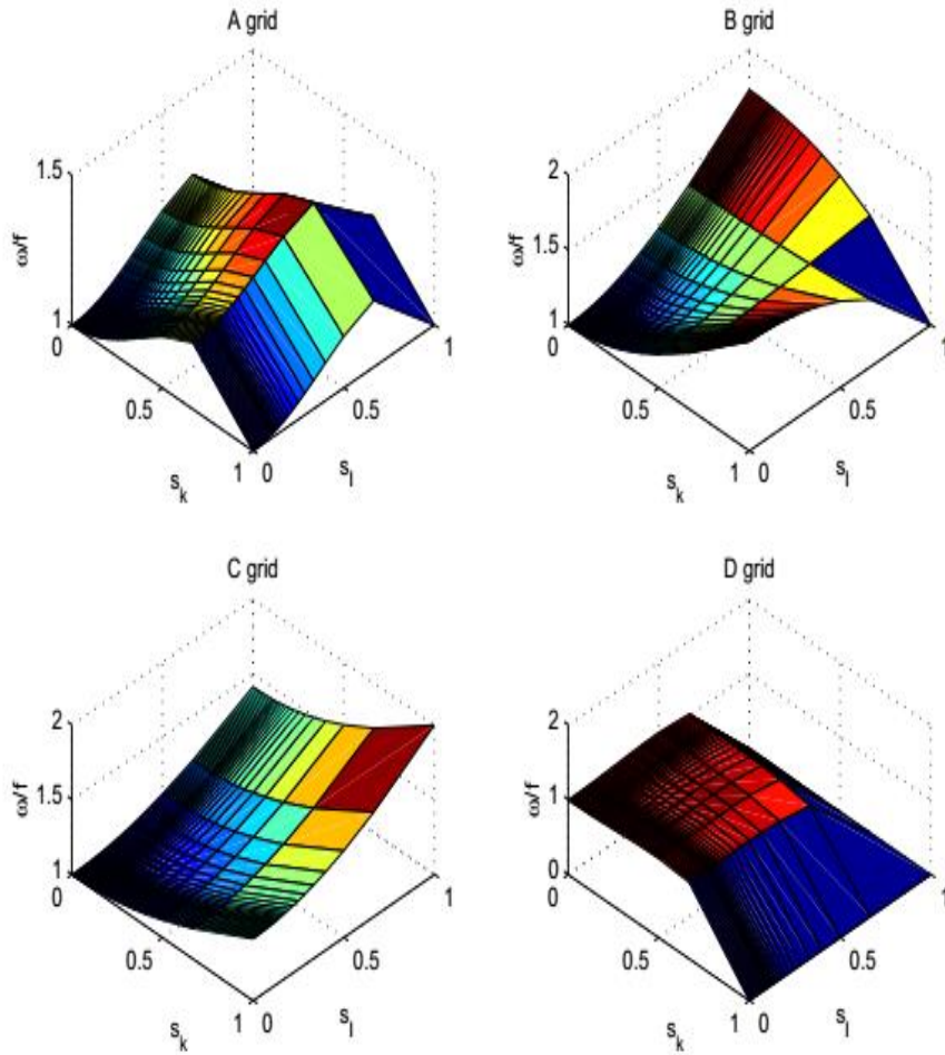
Figure 7.2: Inertia-gravity wave dispersion relations on the Arakawa grids A,B,C and D for coarse resolution. The resolution parameters are r_x = r_y = 0.5 .
