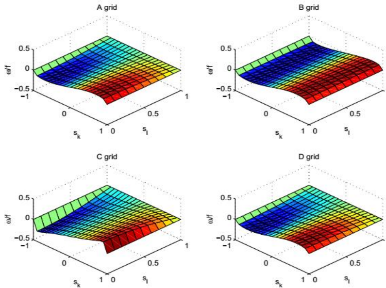
Figure 7.4: Rossby wave dispersion relations on the Arakawa grids A,B,C and D resolving the deformation radius. The resolution parameters are r_x = r_y = 5 .
