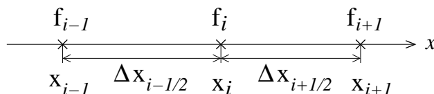
Figure 1: Three point stencil on a variable resolution grid. 20 Marks
