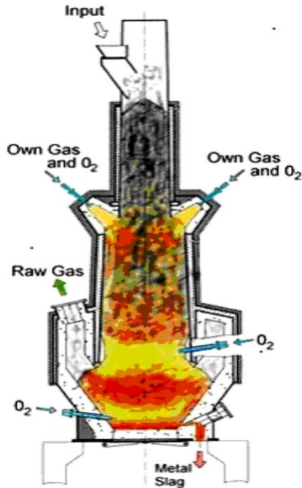
Fig. 1 Process of the pyrolysis system
