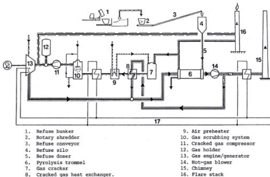
Fig. 2 High temperature gasification process for MSW treatment
