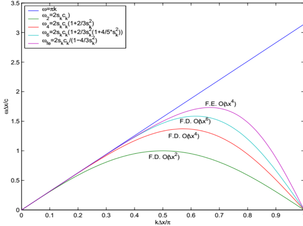
Figure 3.5: Dispersion relations for the O(\Delta x^2) , O(\Delta x^4) and O(\Delta x^6) finite difference methods and the O(\Delta x^4) finite elements method (using the chapeau basis functions).
