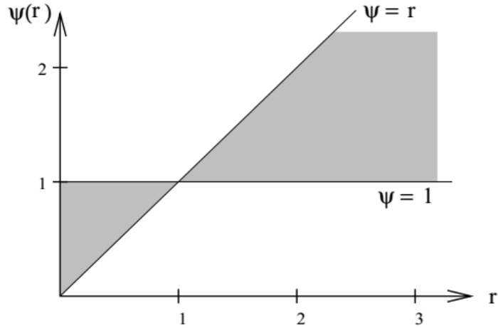
Figure 5.3: The two lines indicate the special limiter functions, \psi(r) = 1 , which yields the Lax-Wendroff flux, and \psi(r) = r which yields the Warming and Beam flux. Since both these schemes are of second order, any linear combination of these schemes is also of second order. The shaded region between them is thus the space where \psi(r) will yield a second order scheme.
