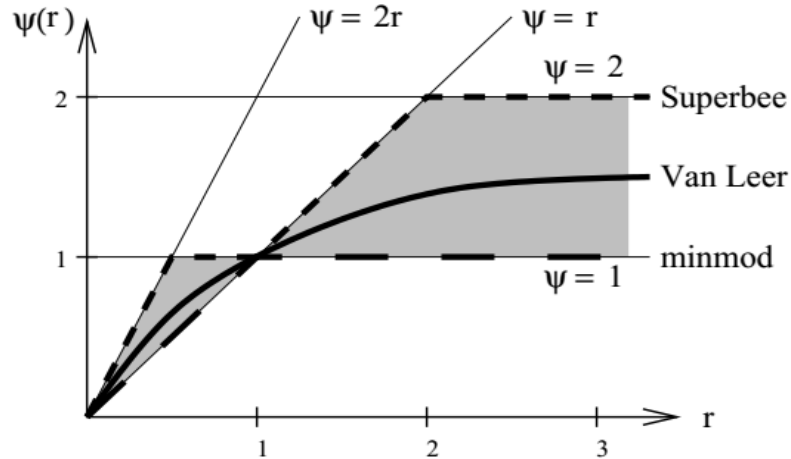
Figure 5.4: The shaded region is the intersection between the TVD region and region of second order accuracy. The short dashed line is the Superbee limiter, the long dash line is the minmod limiter and the solid curve is the Van Leer limiter.
