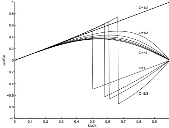
Figure 5.1: The frequency of the FTUS (or “upwind”) scheme for various Courant number C = \frac{\Delta t c}{\Delta x} . C = 1/2 falls on w = k which is the frequency of the continuum.
