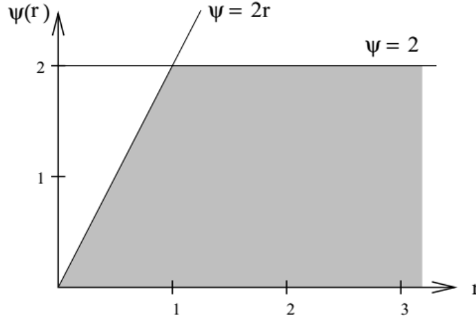
Figure 5.2: The two lines indicate the bounds on the limiter function, \psi(r) given by the constraints for the scheme to be TVD (total variance diminishing).
