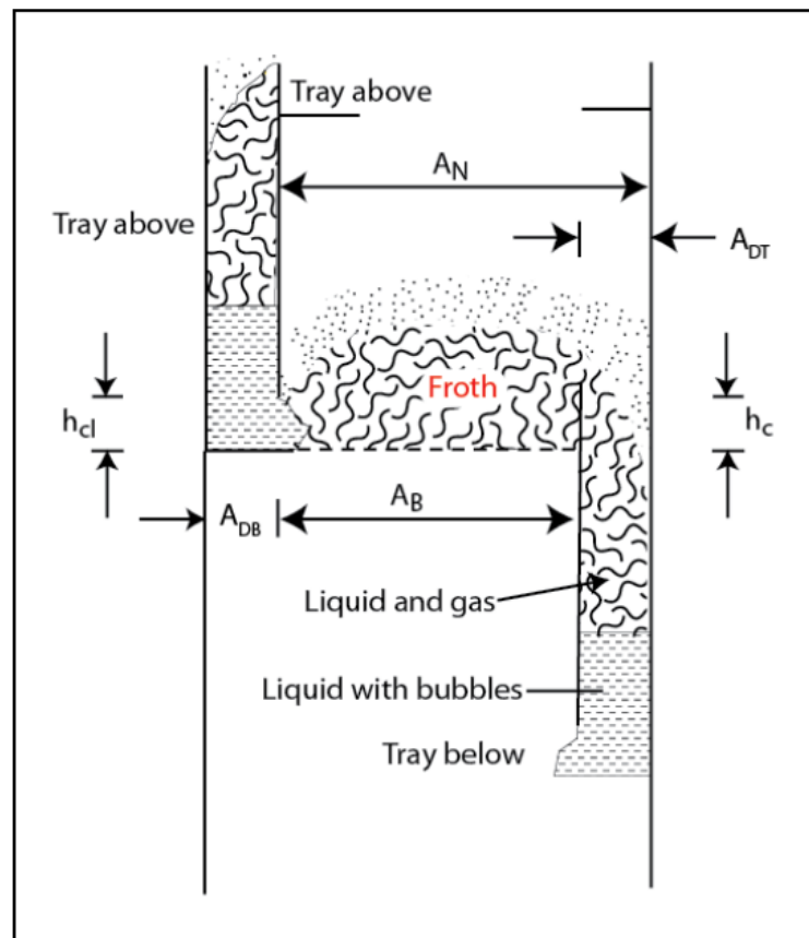
Figure 7.2. Schematic of a tray operating in the froth regime
