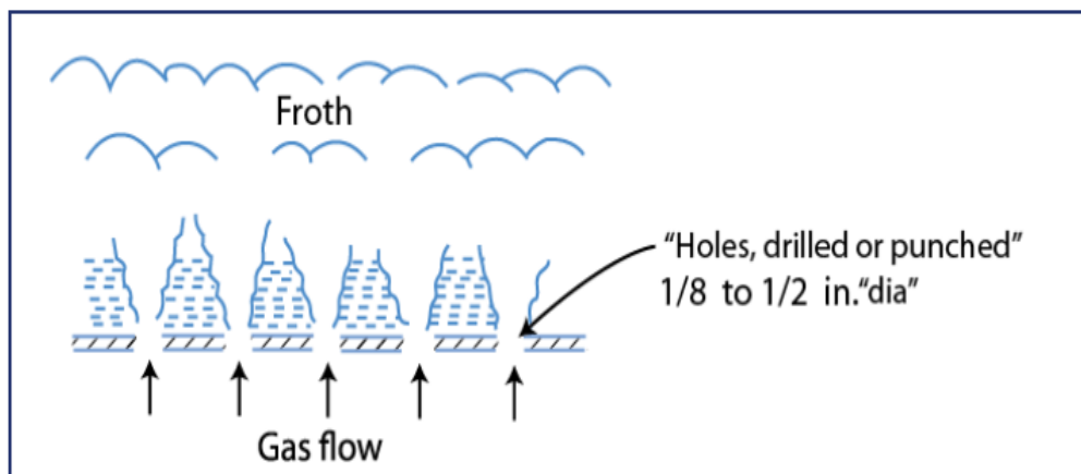
Figure 7.7. Sieve tray
