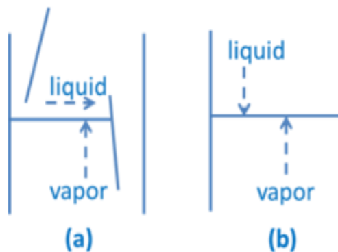
Figure 7.4. Classification of plate types based on flow mode- side view shown: (a) Cross-flow plate, (b): Counterflow plate.
