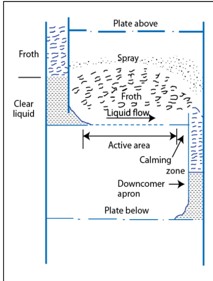
Figure 7.3. Typical cross-flow plate (sieve)
