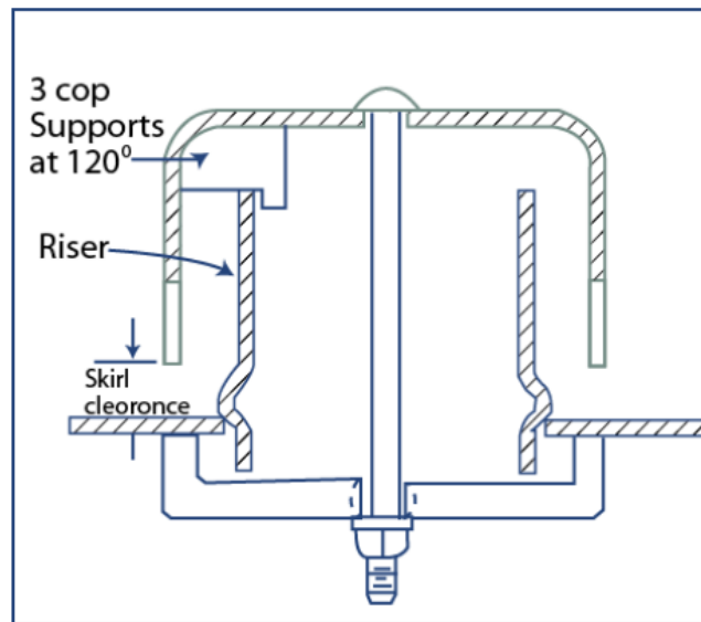
Figure 7.5. Bubble caps
