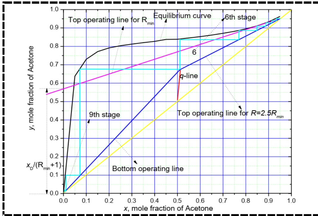
Figure 7.8: McCabe-Thiele construction.
