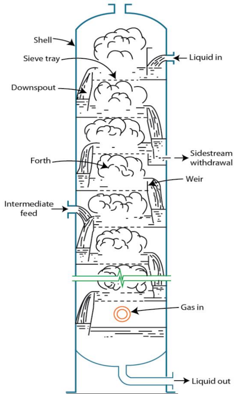
Figure 7.1. Schematic diagram of a plate contractor
