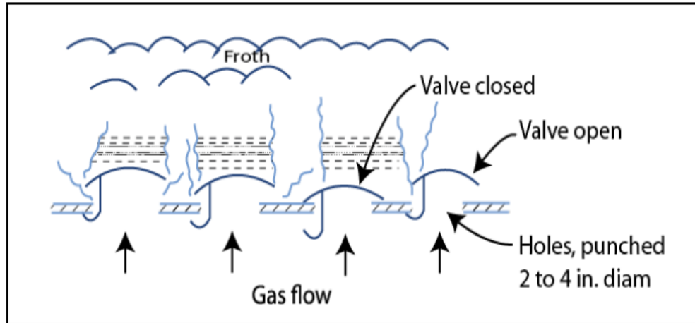
Figure 7.6. Valve tray
