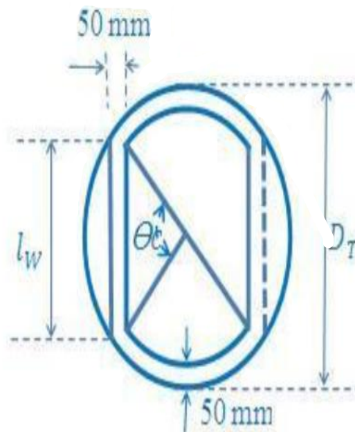
Figure 7.9. Angle subtended by the chord
