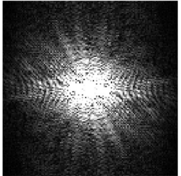
reciprocal space
