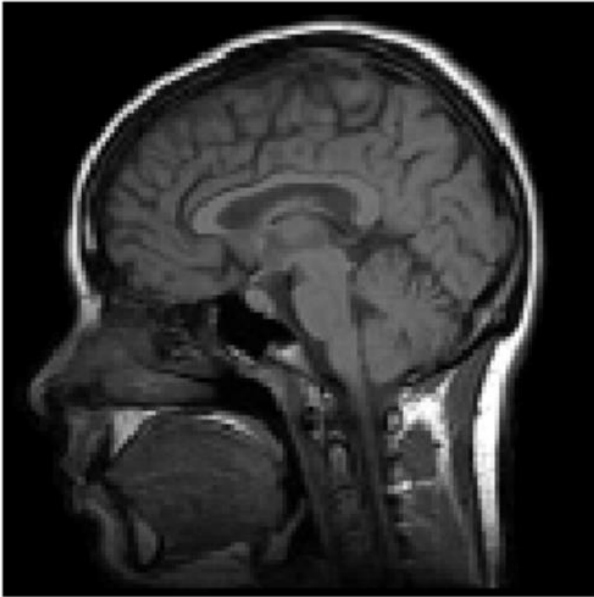
real space
