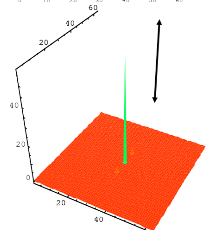
Examples of Fourier transformations for lecture 6
