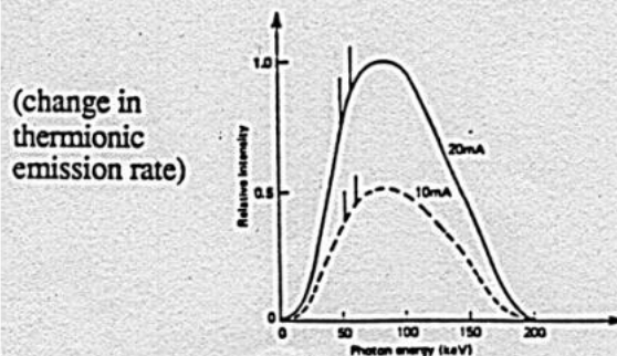
Figure 11.4 Effect of tube current on spectrum
