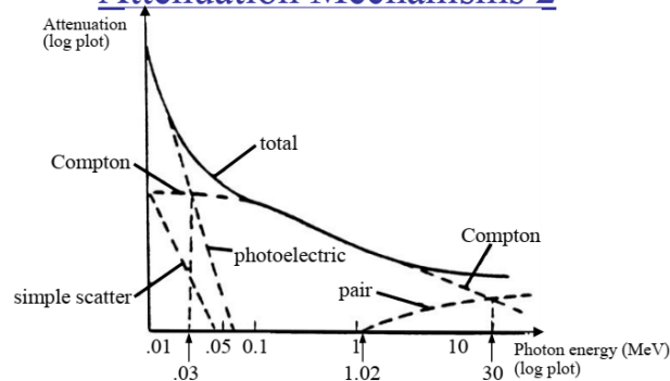
Attenuation mechanisms in water
