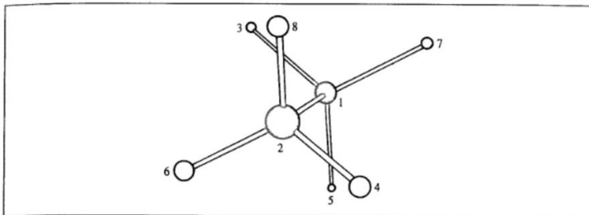
Fig. 1.1 The staggered conformation of ethane
