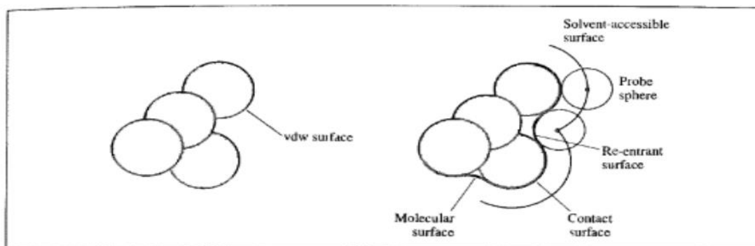
Fig 1.6 The van der Waals (vdw) surface of a molecule corresponds to the outward-facing surfaces of the van der Waals spheres of the atoms. The molecular surface is generated by rolling a spherical probe (usually of radius 1.4 Å to represent a water molecule) on the van der Waals surface. The molecular surface is constructed from contact and re-entrant surface elements. The centre of the probe traces out the accessible surface.
