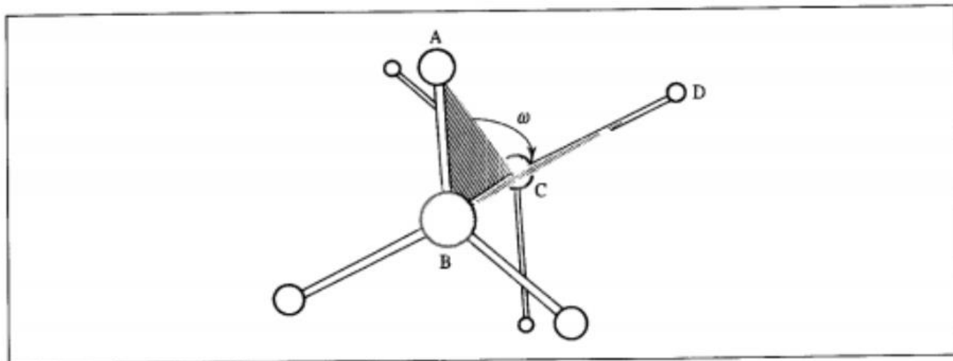
Fig. 1.2 A torsion angle A-B-C-D is defined as the angle between the planes A, B, C and B, C, D. A torsion angle can vary through 360° although the range -180° to +180° is most commonly used. We shall adopt the IUPAC definition of a torsion angle in which an eclipsed conformation corresponds to a torsion angle of 0° and a trans or anti conformation to a torsion angle of 180°. The reader should note that this may not correspond to some of the definitions used in the literature, where the trans arrangement is defined as a torsion angle of 0°. If one looks along the bond B-C, then the torsion angle is the angle through which it is necessary to rotate the bond AB in a clockwise sense in order to superimpose the two planes, as shown.
